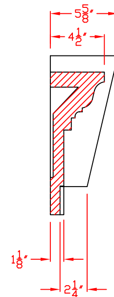
SEC :A-A
